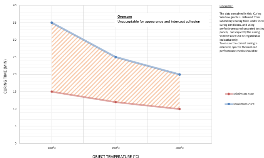
Interpon D2525 Texture ISR - curing window
